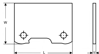
Leuco Superprofiler System*
